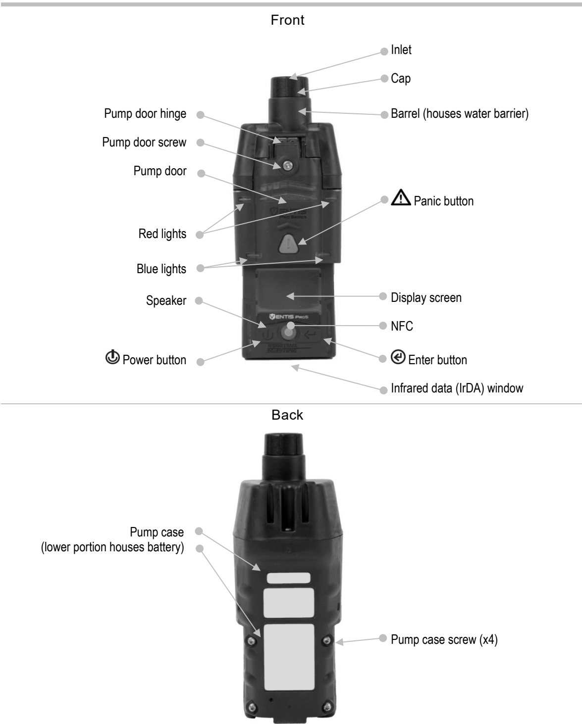
Figure 3.1.B Hardware overview aspirated instrument
