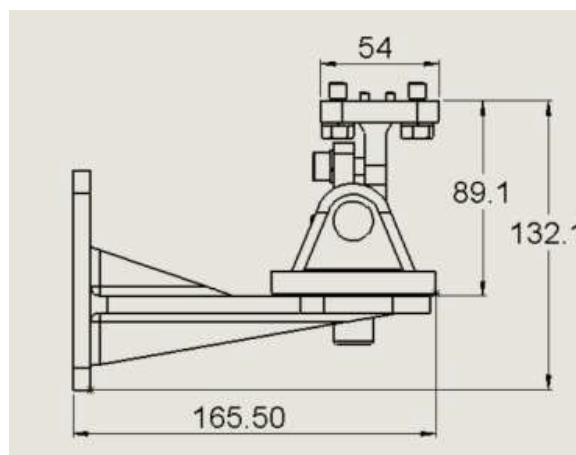
Figure 12 : Tilt mount base – Side View
