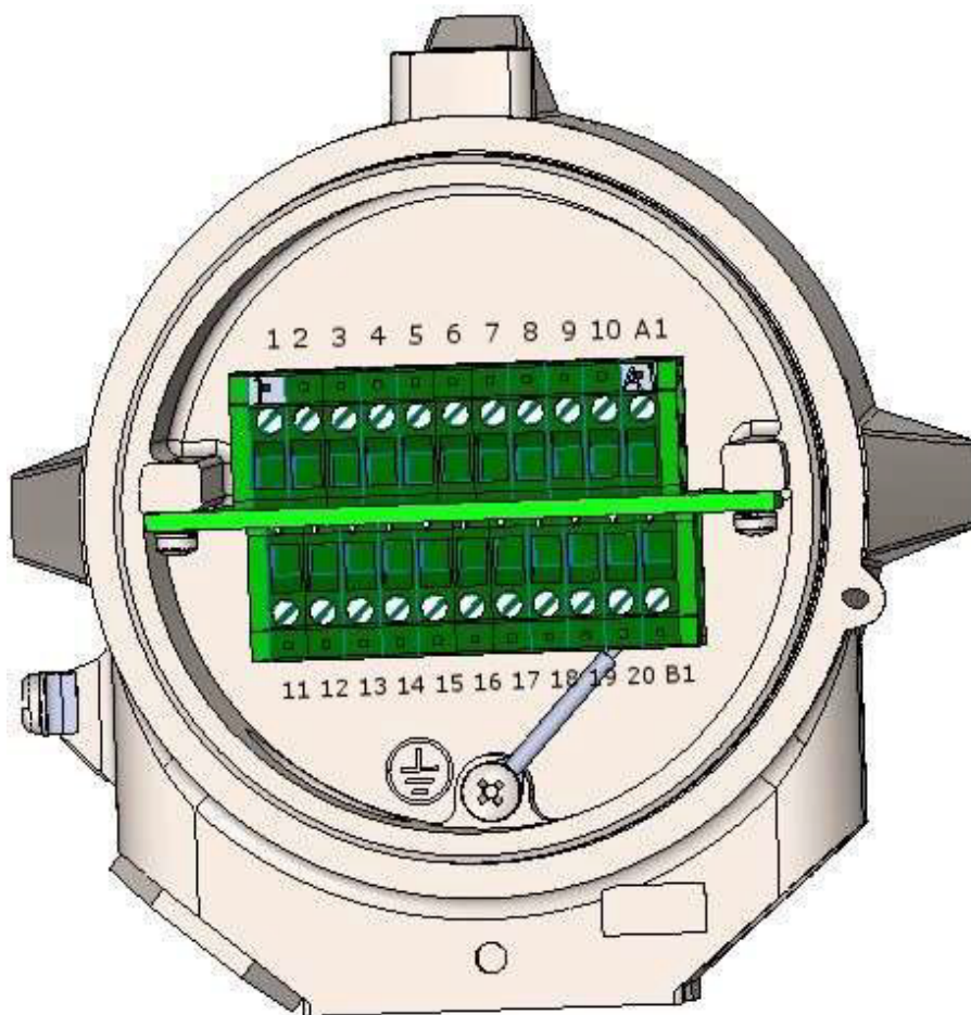
Figure 14 : Terminal view
