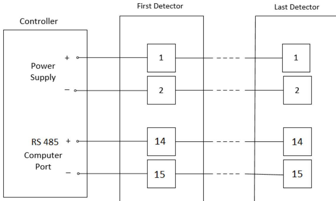
Figure 20 : RS-485 Networking
