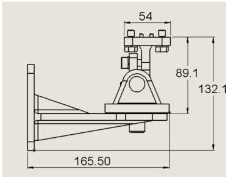
Figure 12 : Tilt mount base – Side View
